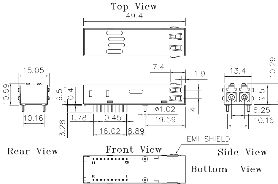
TRSL-5380WE-CXX0G / TRSL-5380CWE-CXX0G
