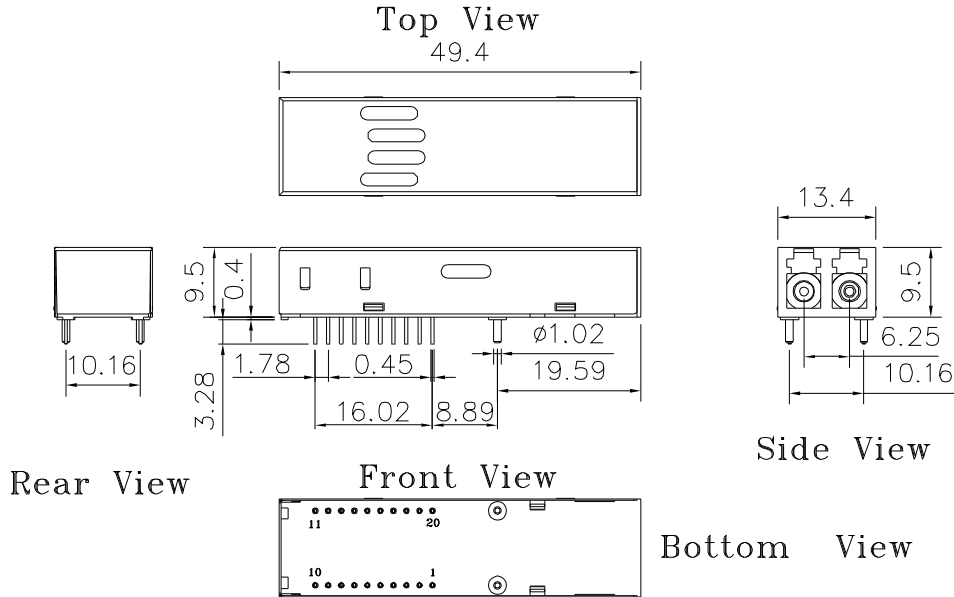
TRSL-5380W-CXX0G / TRSL-5380CW-CXX0G
